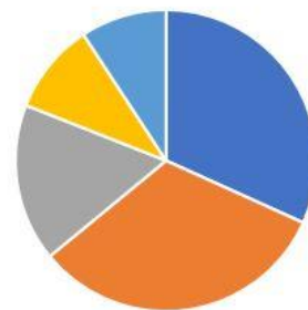
Starts by Parliamentary Constituency
